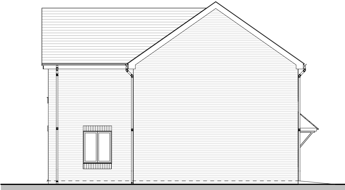
Side Left Elevation
