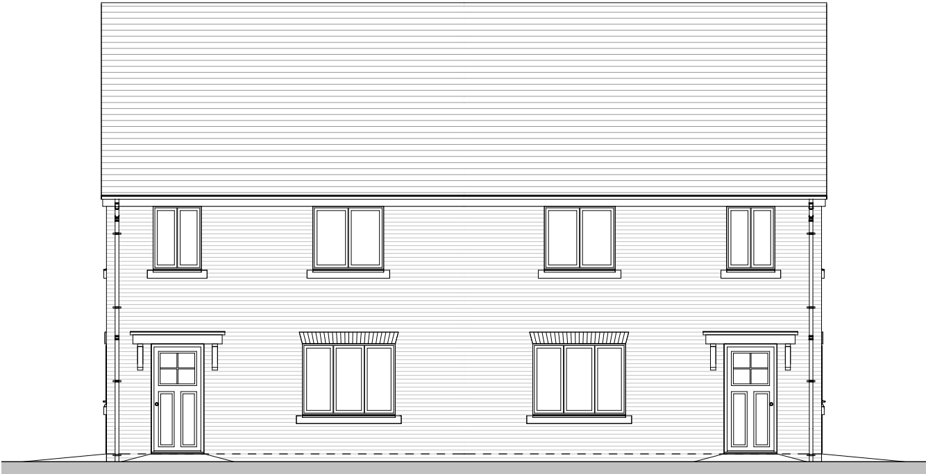
Front Elevation
