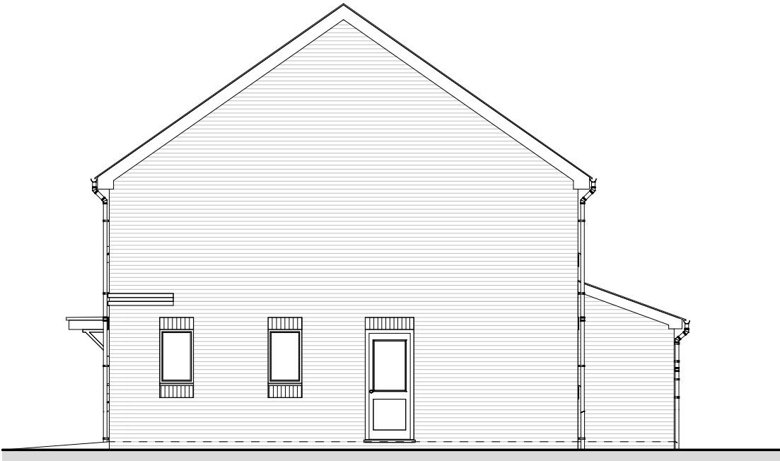
Side Right Elevation
