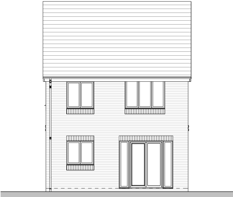
Rear Elevation
