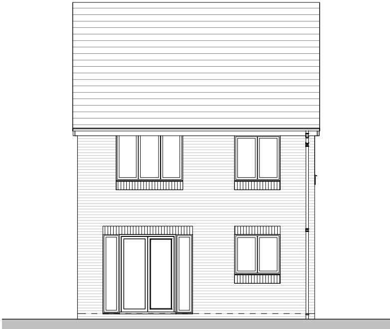
Rear Elevation
