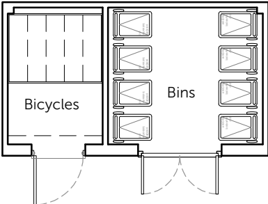
Floor Plan
