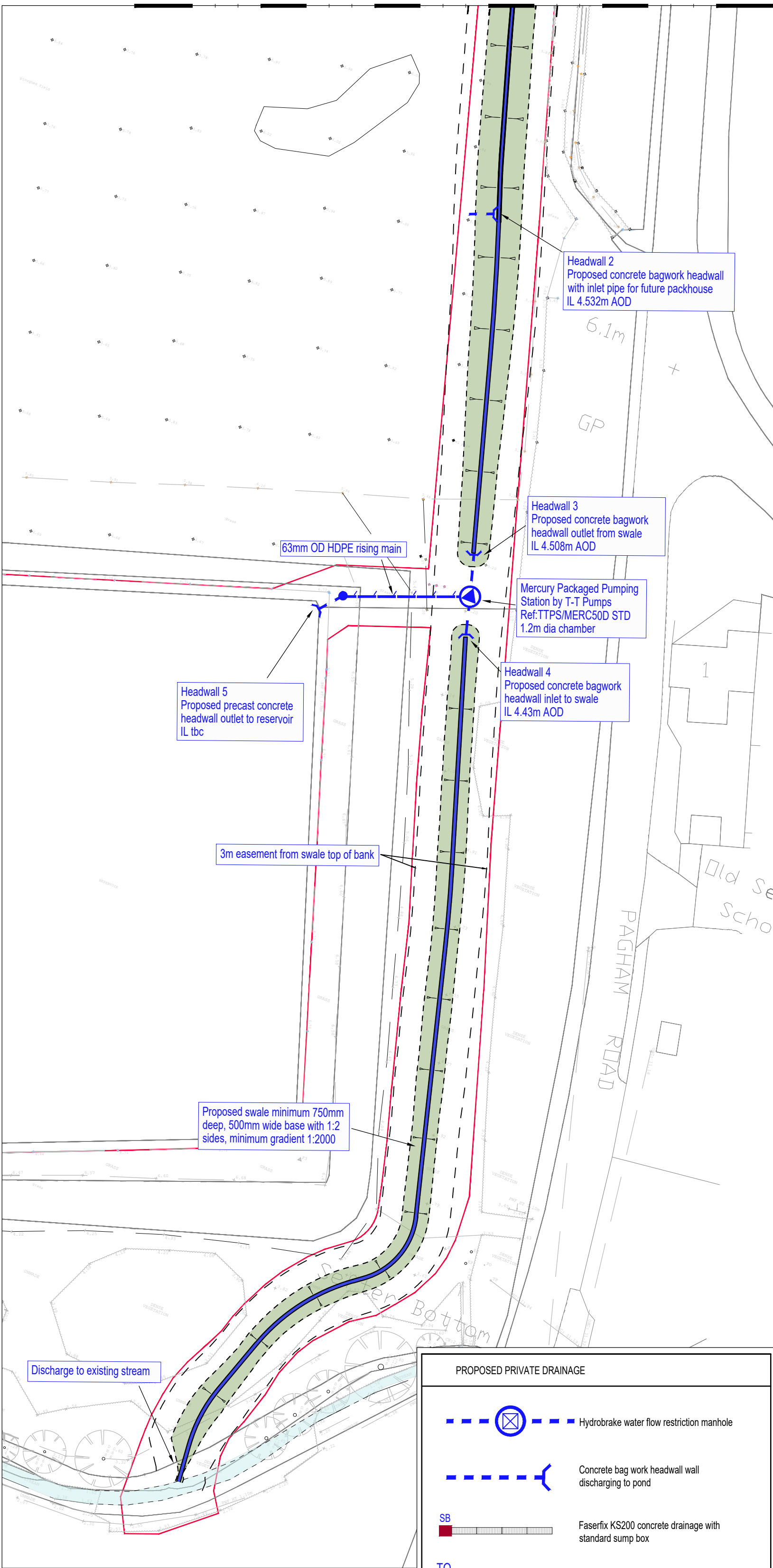
CUTLINE - FOR CONTINUATION OF SWALE SEE MAIN PLAN
