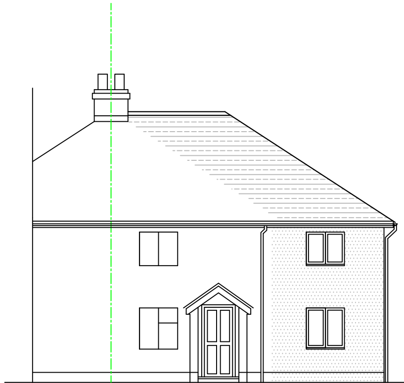
Proposed Front Elevation (North)
