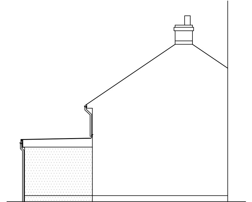
Proposed Side Elevations (East)
