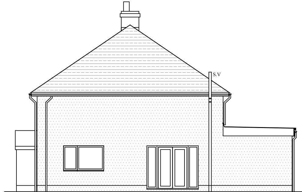
Proposed Side Elevations (West)
