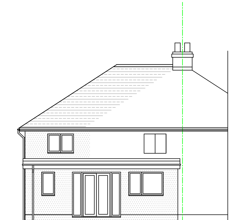
Proposed Rear Elevation (South)
