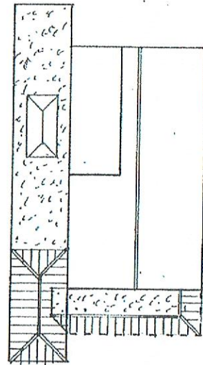
Approved single story roof Plan 1:200
