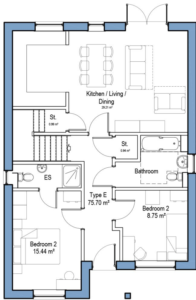
House Type E Ground Floor Plan 3 Bed / 3 Person Bungalow GIA: 105m²
