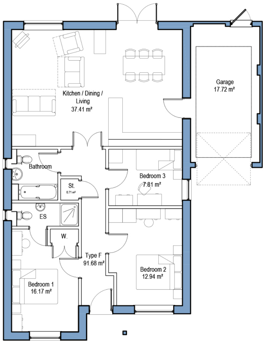
House Type F Ground Floor Plan 3 Bed / 5 Person Bungalow GIA: 91.7m²
