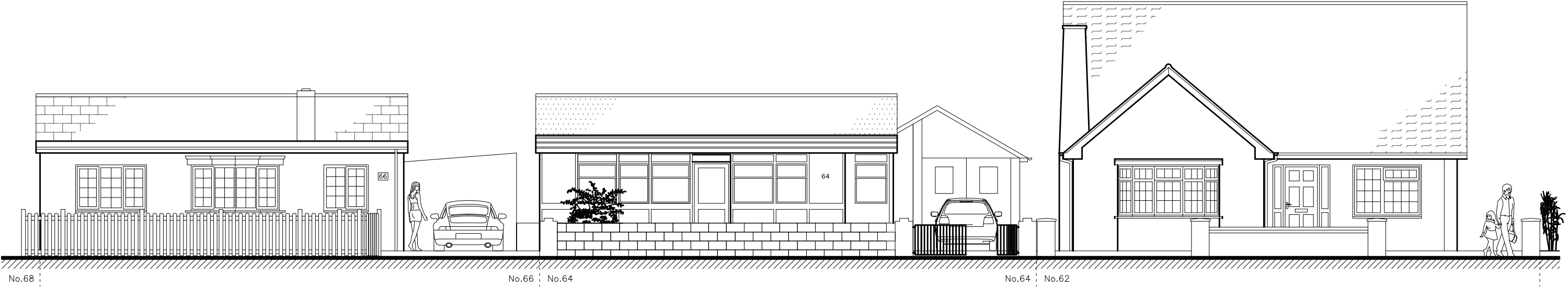
EXISTING SOUTH-EAST STREET SCENE REF. NO.: BD535 ESE01-1
