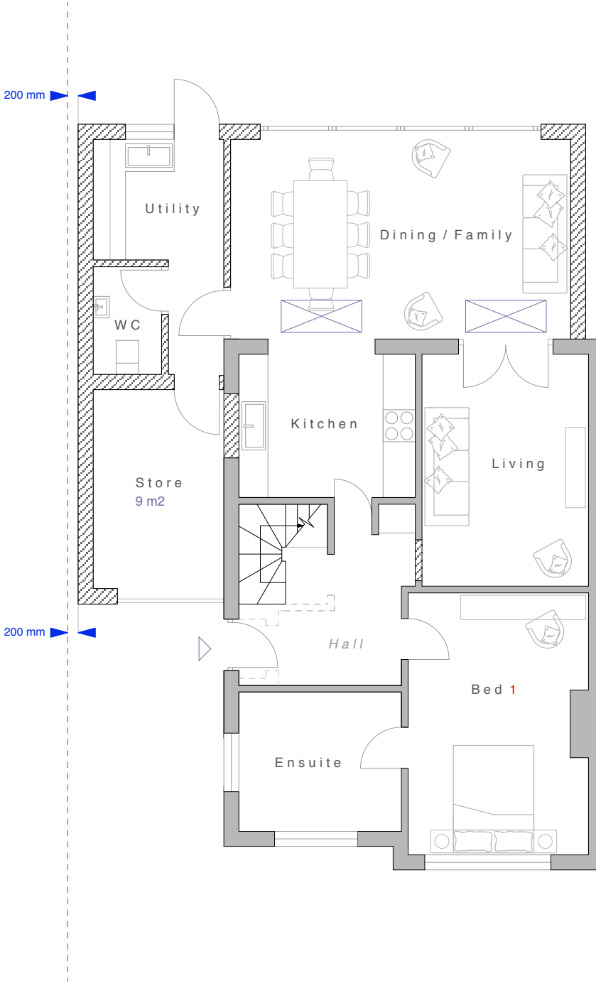
Proposed GF Plan at 1:100 scale
