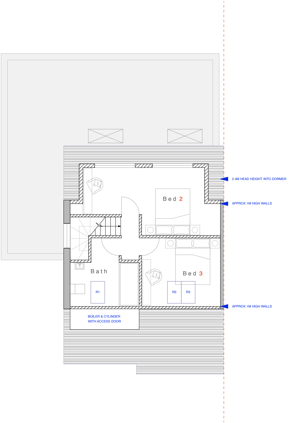
Proposed FF Plan at 1:100 scale
