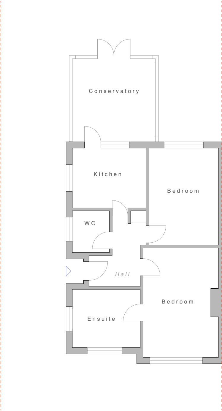
Existing GF Plan at 1:100 scale
