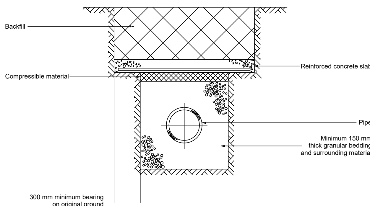
FIGURE B.24 TYPICAL INSPECTION CHAMBER DETAIL - TYPE E
