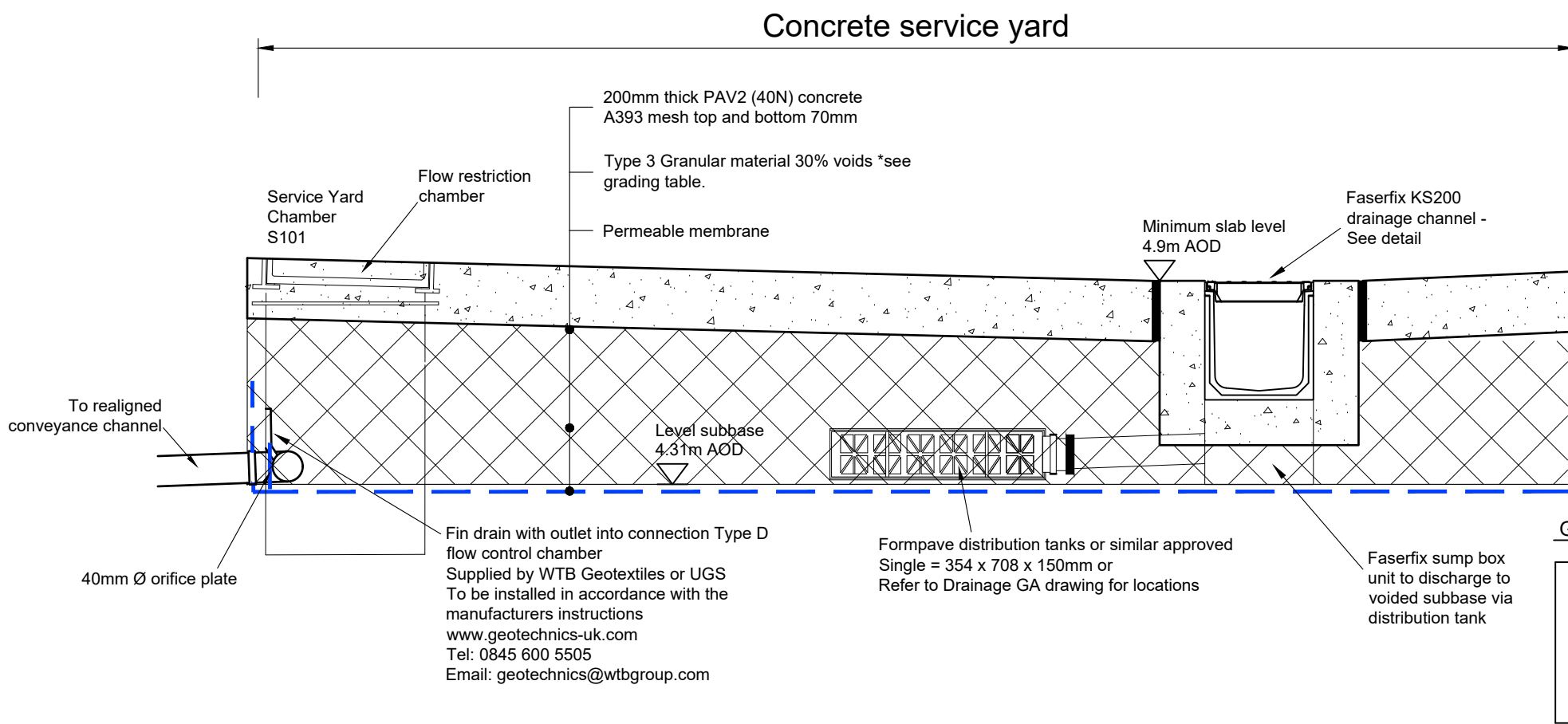
CONCRETE YARD VOIDED SUBBASE CONSTRUCTION DETAIL (Scale 1:20)
