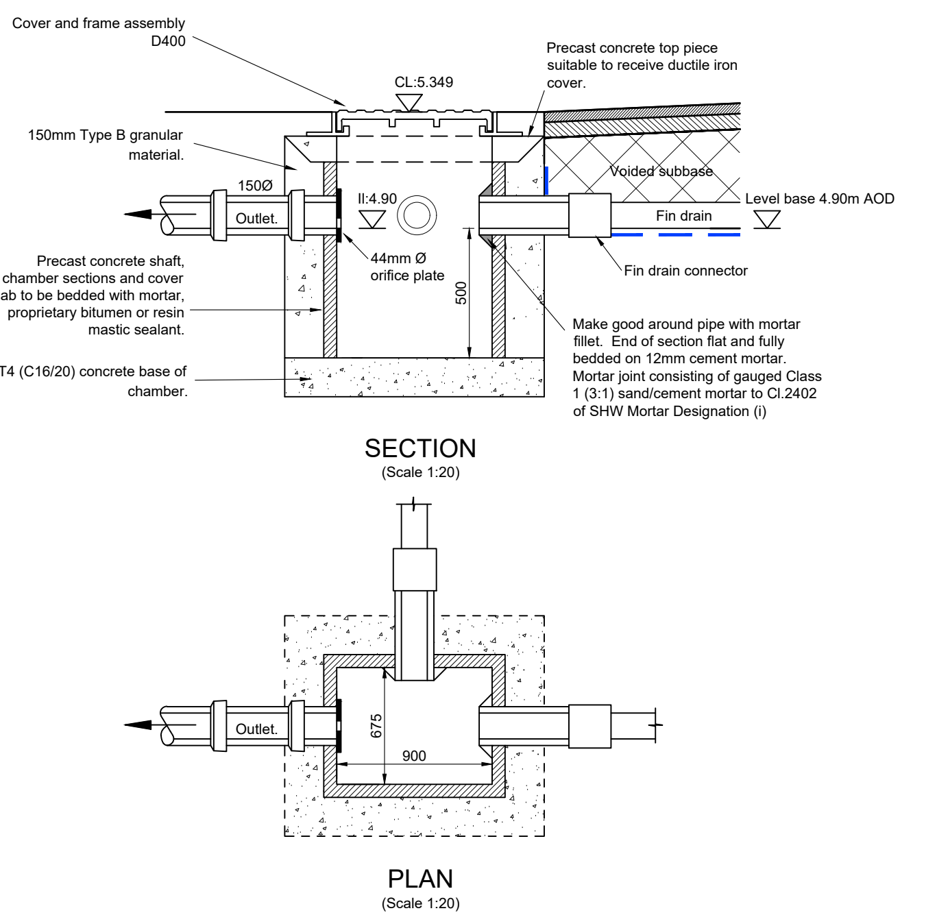
S102 FLOW RESTRICTION MANHOLE CONSTRUCTION DETAILS
