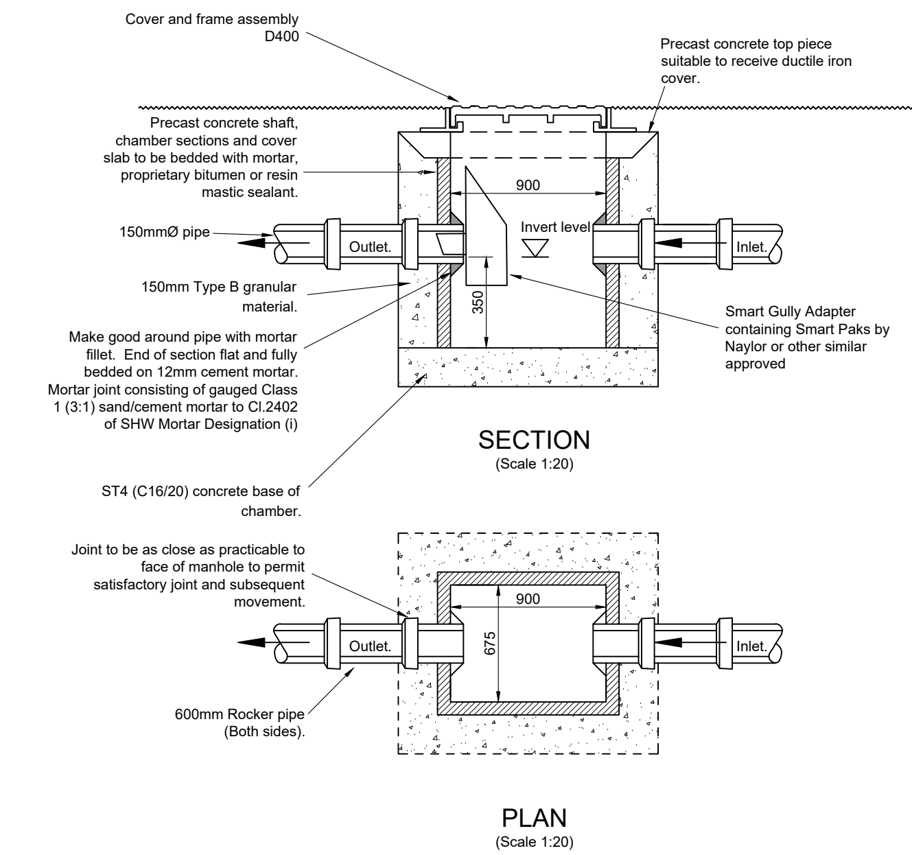
SMART SPONGE CHAMBER CONSTRUCTION DETAILS
