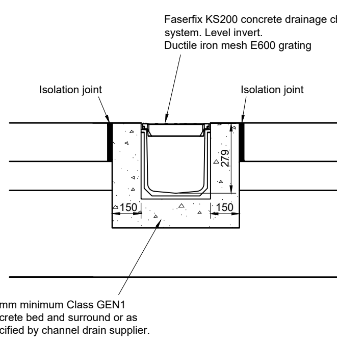
FASERFIX KS200 DRAINAGE CHANNEL DRAIN DETAIL (Scale 1:20)
