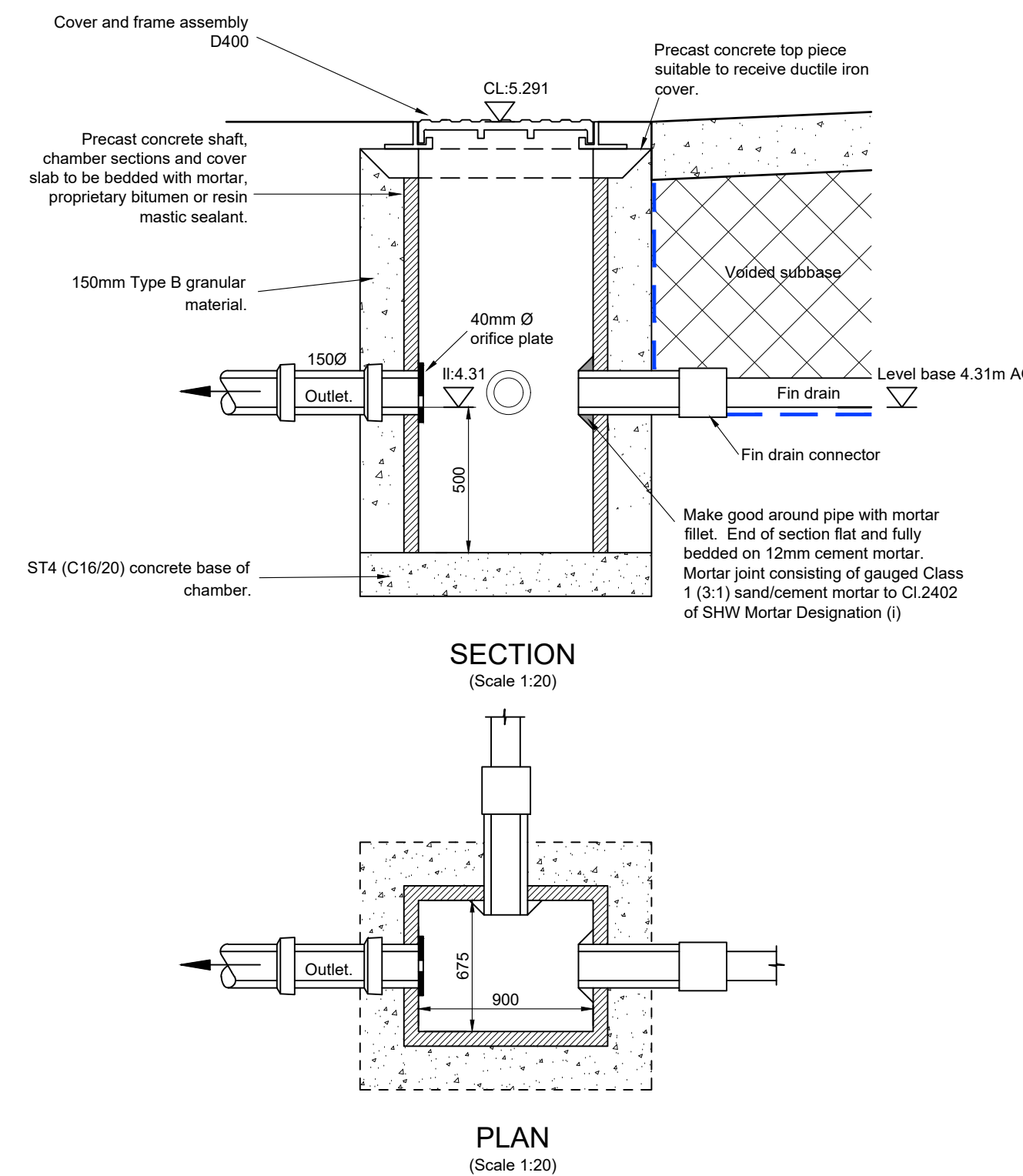
S101 FLOW RESTRICTION MANHOLE CONSTRUCTION DETAILS
