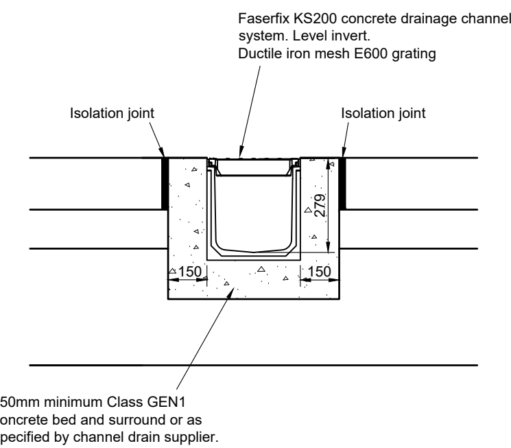
FASERFIX KS200 DRAINAGE CHANNEL DRAIN DETAIL (Scale 1:20)
