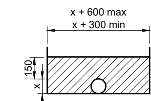
CLASS D PIPE BEDDING
