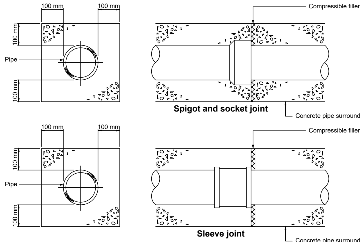
FIGURE B.28 JOINTS FOR CONCRETE ENCASED PIPES
