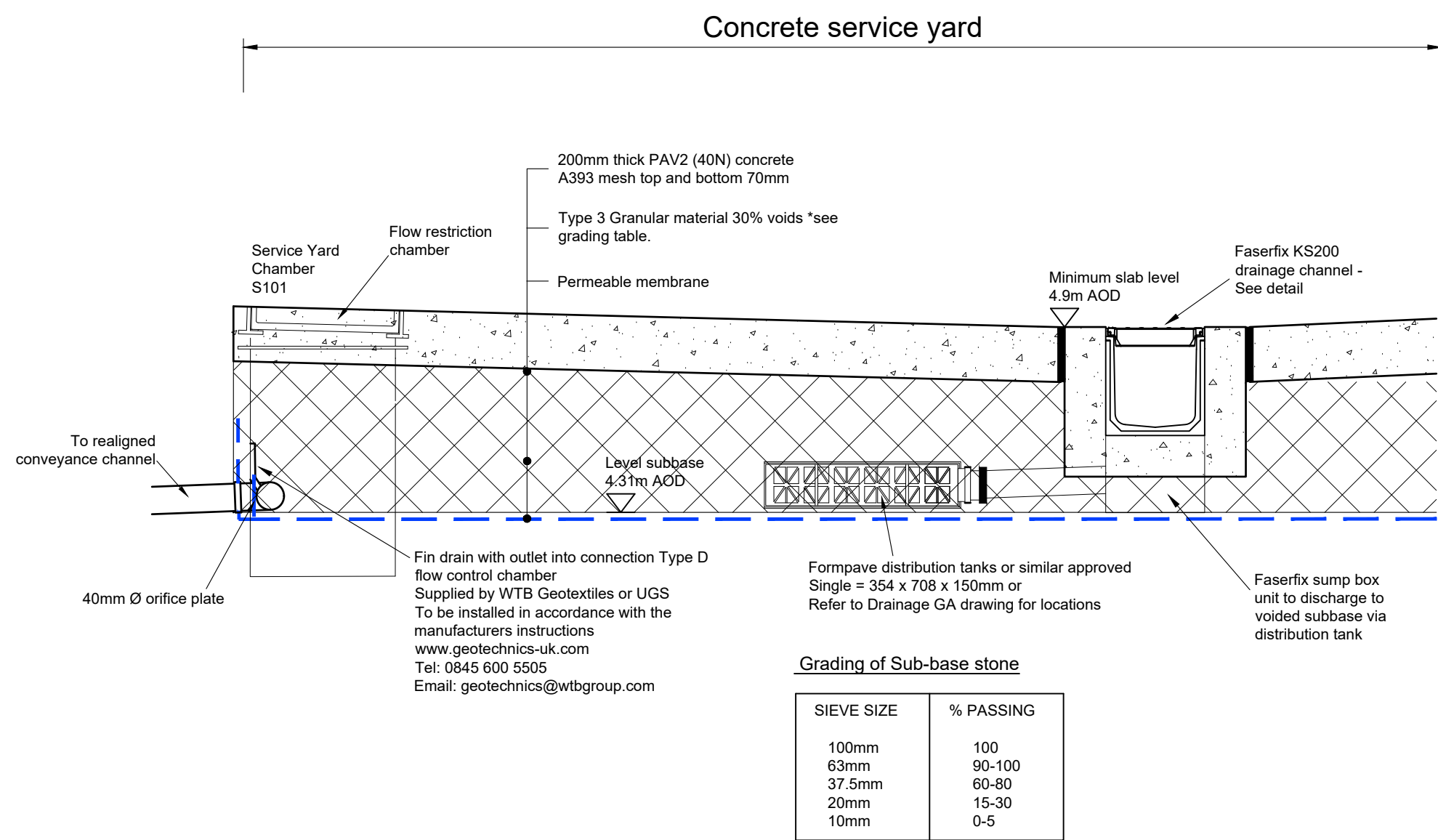
CONCRETE YARD VOIDED SUBBASE CONSTRUCTION DETAIL (Scale 1:20)
