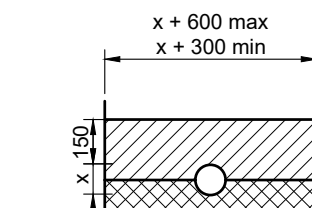
CLASS B PIPE BEDDING
