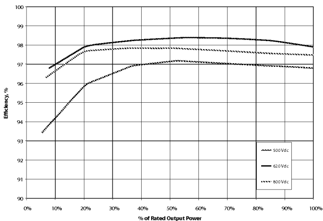
TRIO-20.0-TL-OUTD
