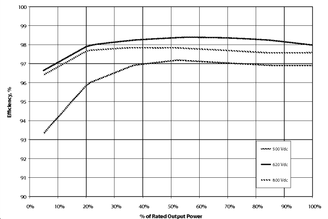
TRIO-27.6-TL-OUTD
