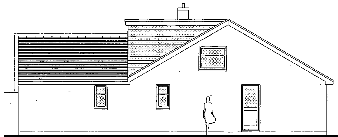
Proposed North Elevation at 1:100 scale
