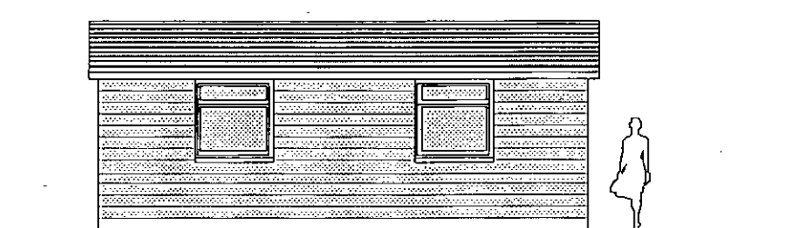
Proposed South Elevation at 1:100 scale
