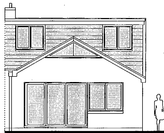
Proposed East Elevation at 1:100 scale
