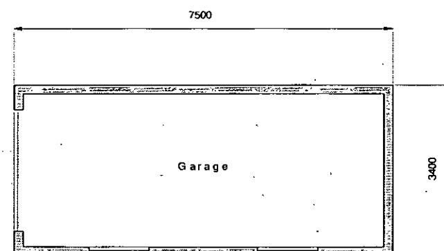
Proposed Garage Plan at 1:100 scale
