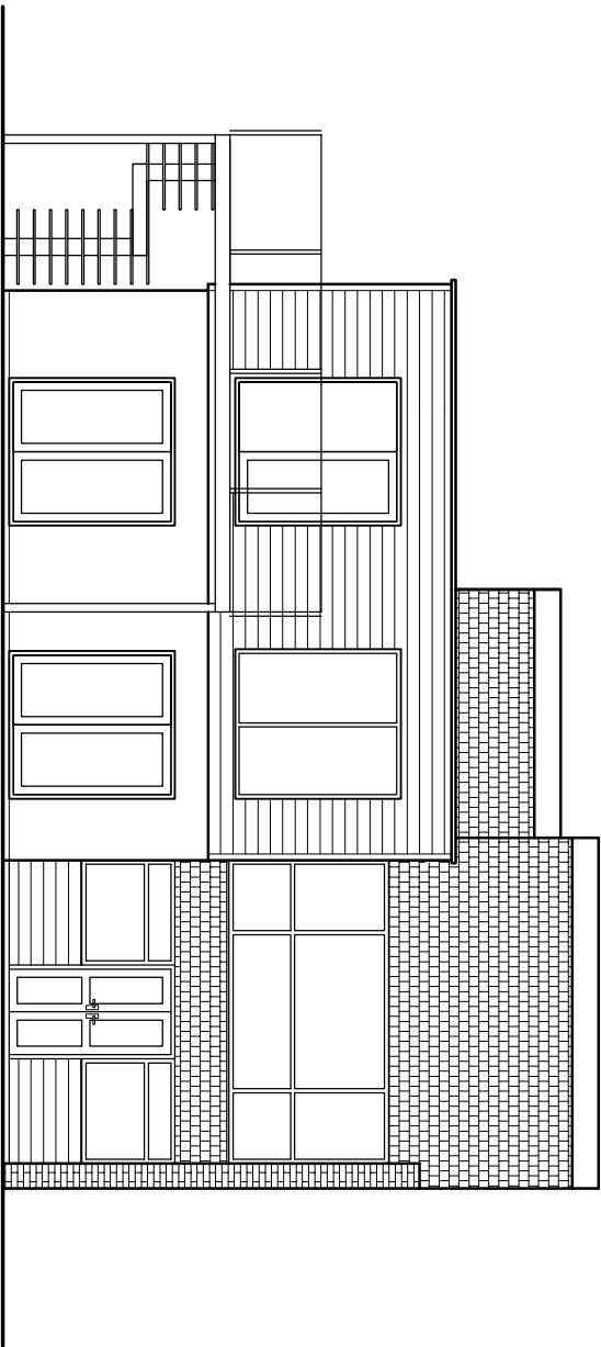
South (rear)
