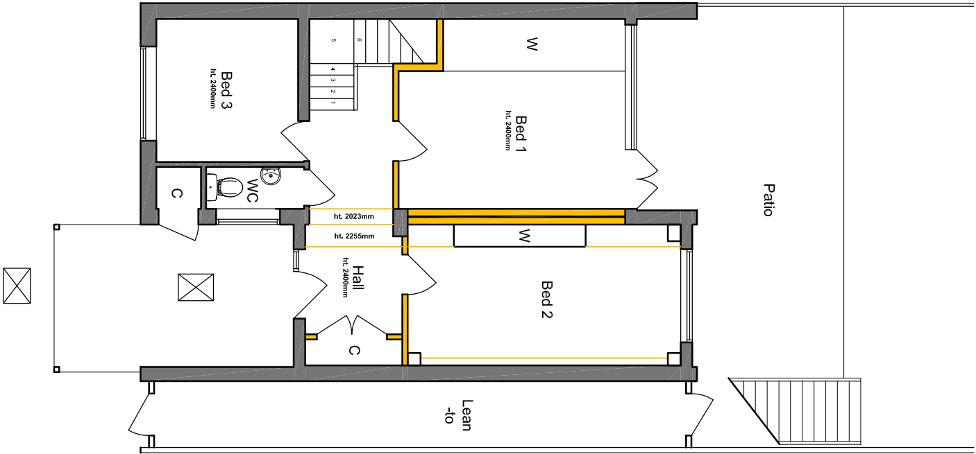
Ground floor
