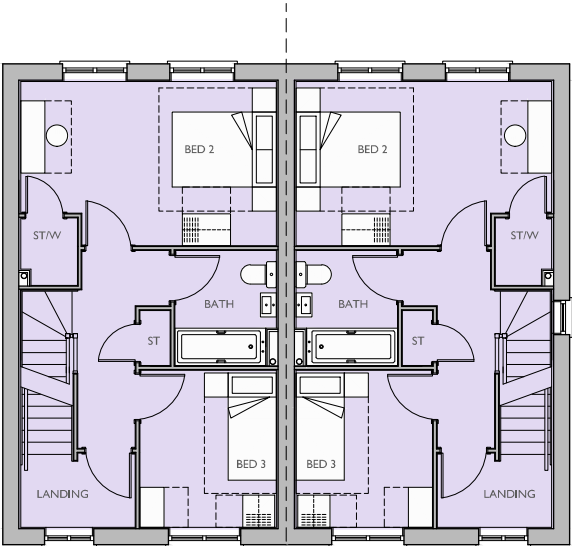
FIRST FLOOR PLAN + Window to Plot 150 Only
