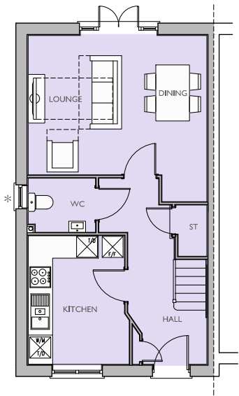
GROUND FLOOR PLAN * OBSCURE GLAZED WINDOW
