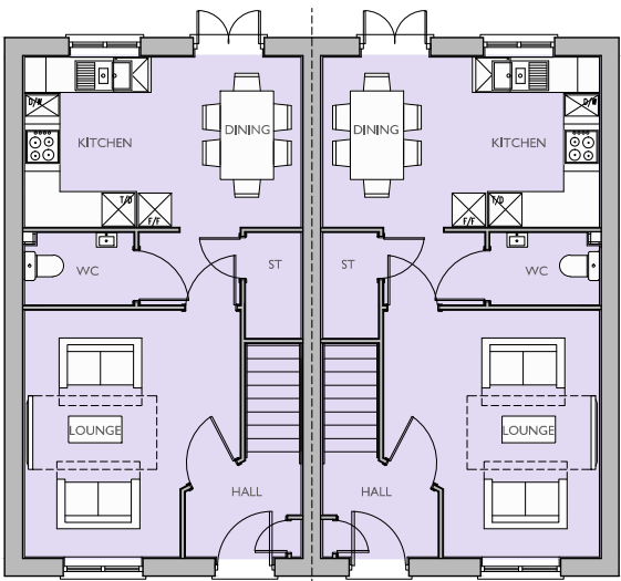
GROUND FLOOR PLAN * OBSCURE GLAZED WINDOWS
