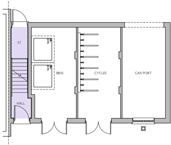
GROUND FLOOR PLAN ■ BLACKENED GLASS WINDOW
