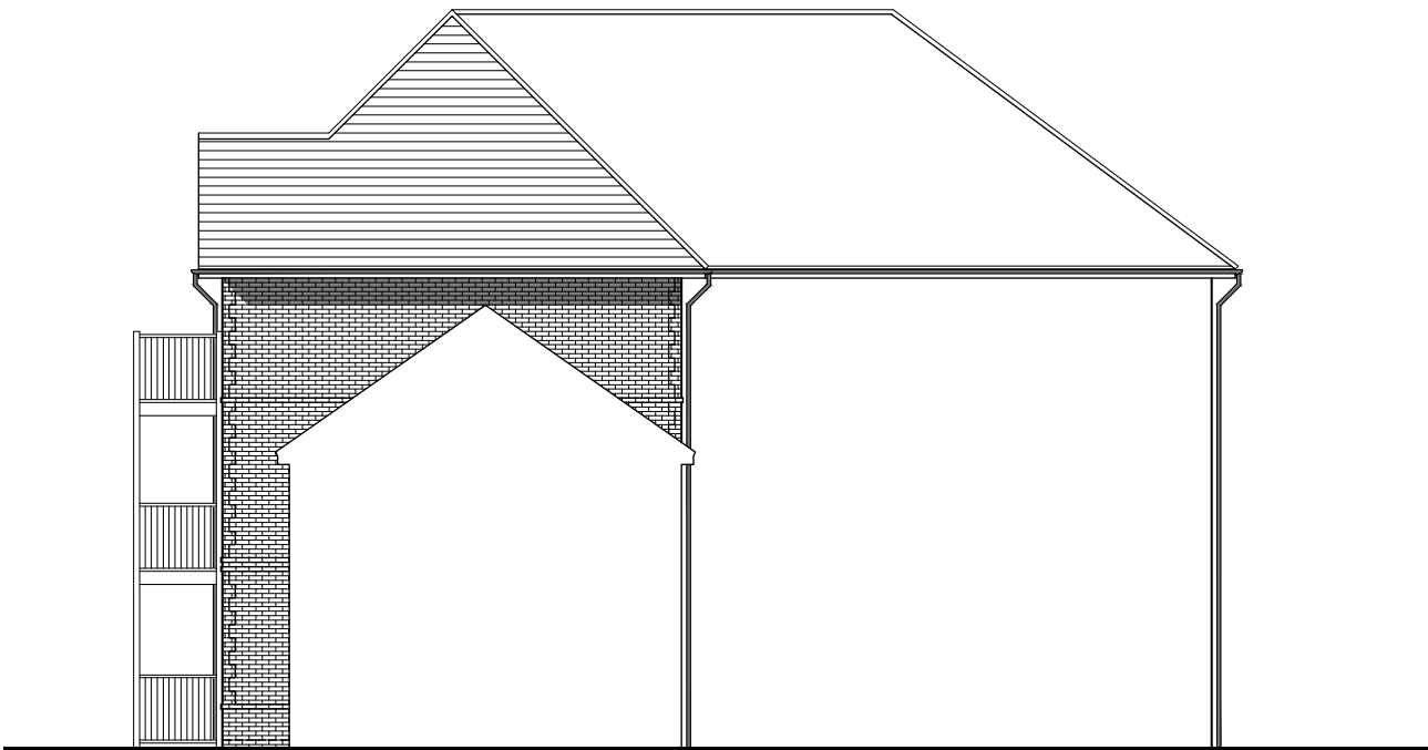
SIDE ELEVATION
