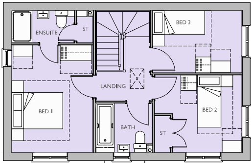
FIRST FLOOR PLAN *: OBSCURE GLAZED WINDOW
