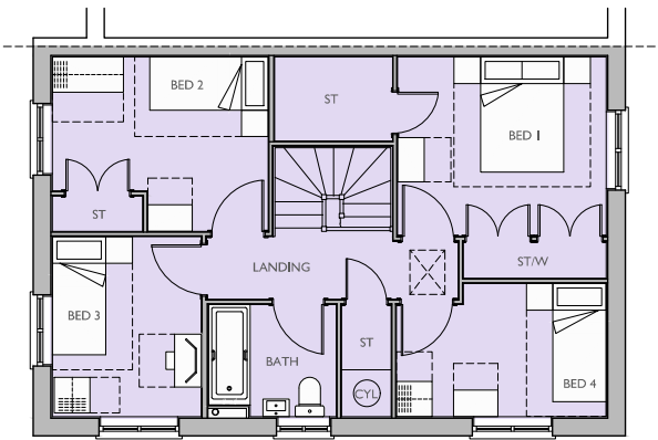
FIRST FLOOR PLAN * OBSCURE GLAZED WINDOW
