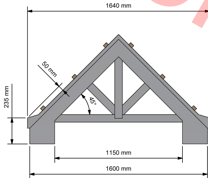
Front Elevation ( 1 : 20 )
