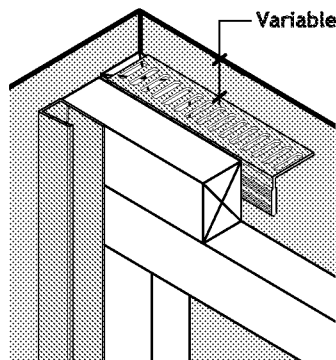
Fix 1 part trims, first part of 2 part trims & vented starter trims. Refer to Diagrams 5, 6, 7 & 8.
