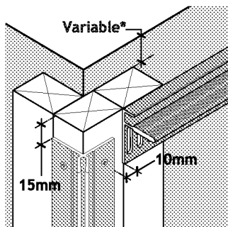
Fix 1 part trims, first part of 2 part trims & vented starter trims. Refer to Diagrams 5, 6, 7 & 8.
