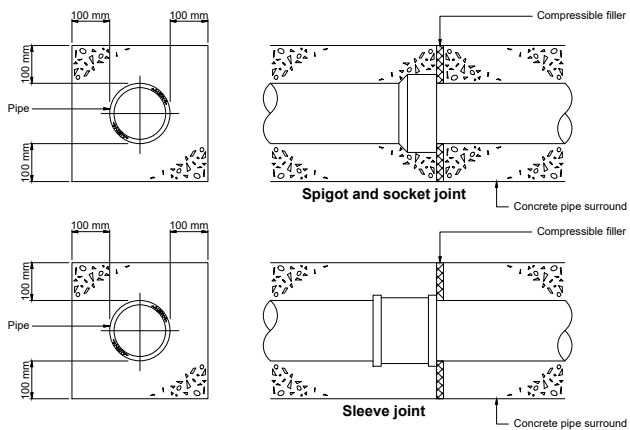
FIGURE B.28 JOINTS FOR CONCRETE ENCASED PIPES
