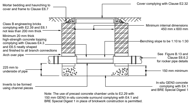
FIGURE B.24 TYPICAL INSPECTION CHAMBER DETAIL - TYPE E Depth from cover level to soffit of pipe up to 1 m Rigid material construction
