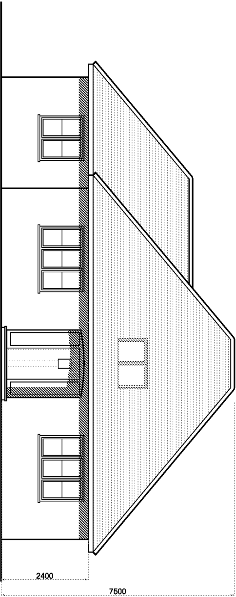
Proposed Front Elevation - NW
