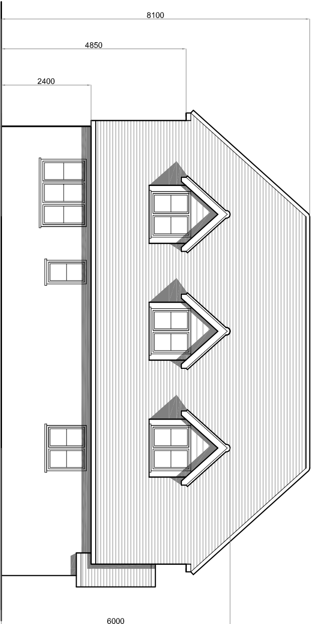
Proposed Side Elevation - NW
