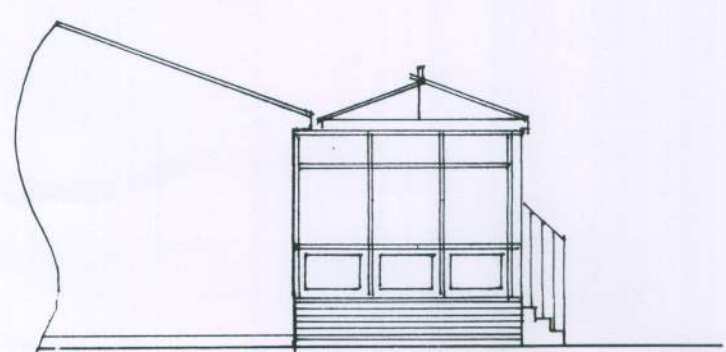
south 1 : 100
