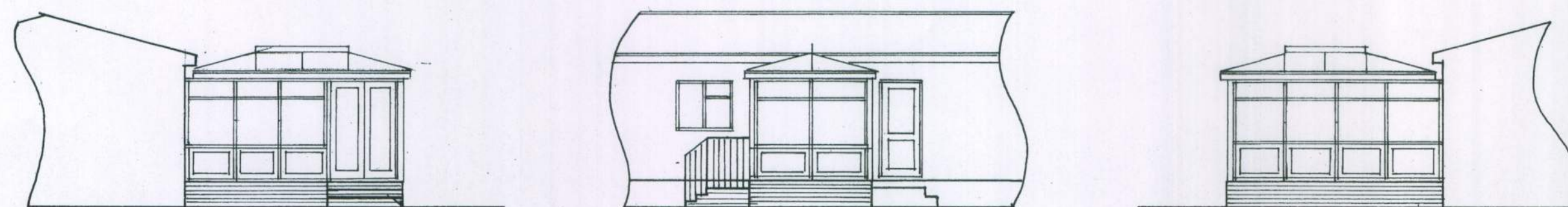
south 1 : 100
