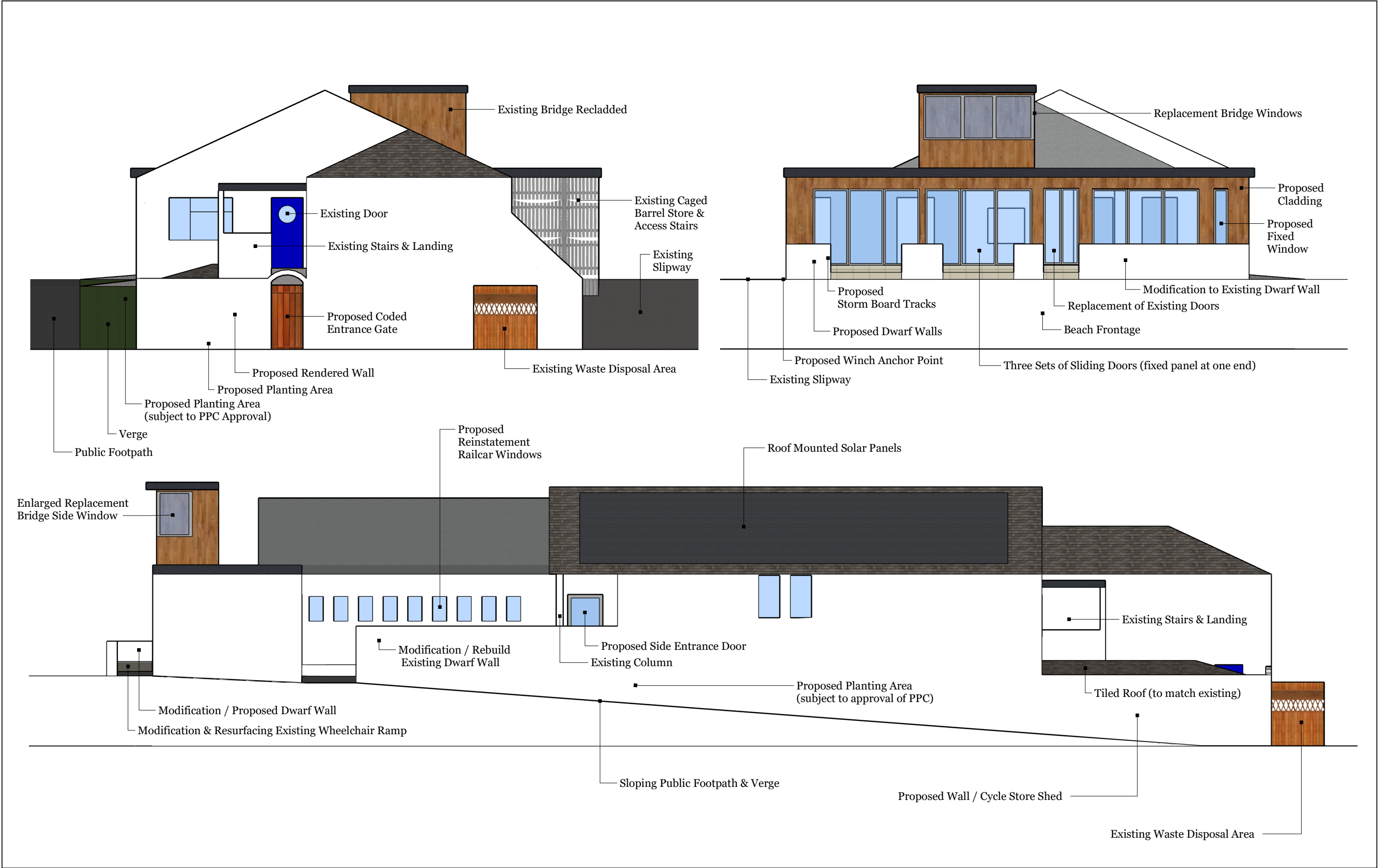
Proposed North, South & East Elevations (NOTE: West Elevation As Existing)
