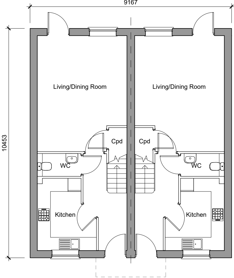
Type Baker Ground Floor Plan 2-Bedroom House 81.3sqm / 876sqft GIA [to finishes] Plots 43, 44
