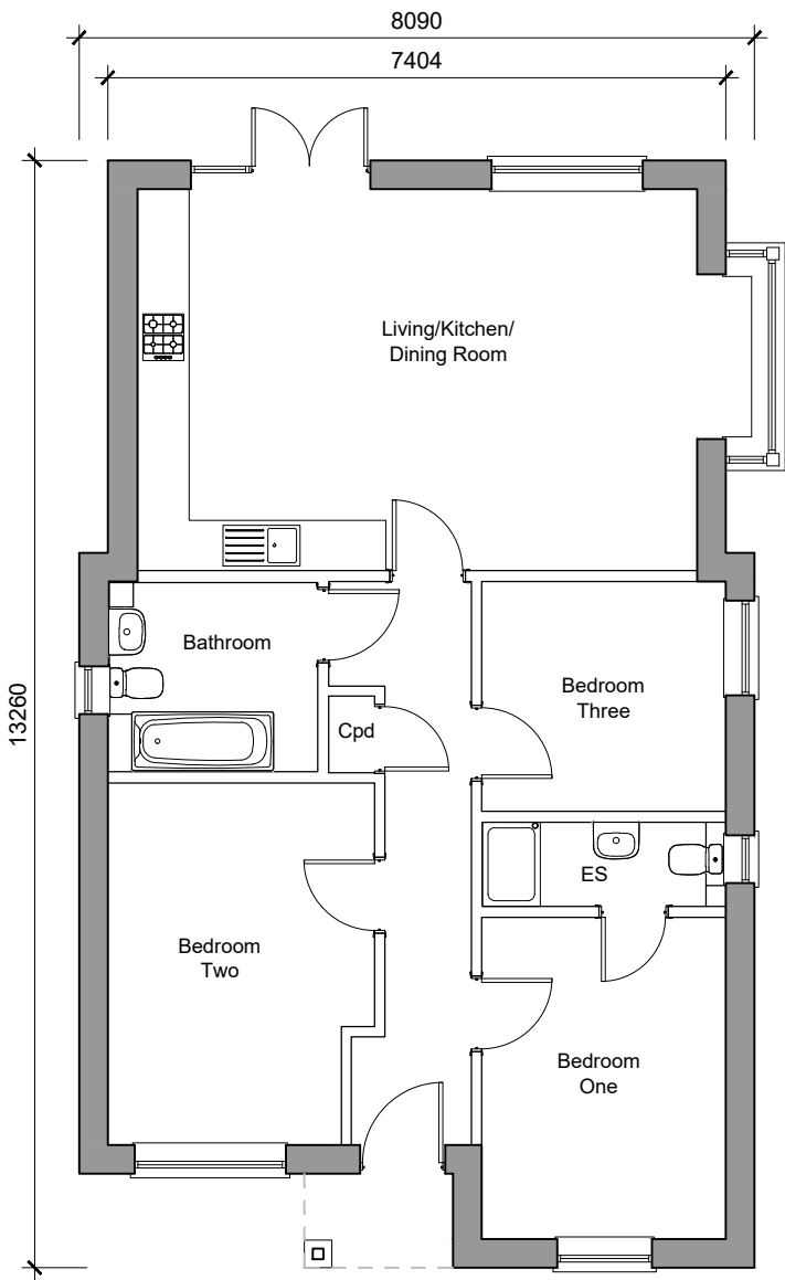
Type Bungalow Ground Floor Plan 3-Bedroom Bungalow 85.9sqm / 925sqft GIA [to finishes] Plots 83
