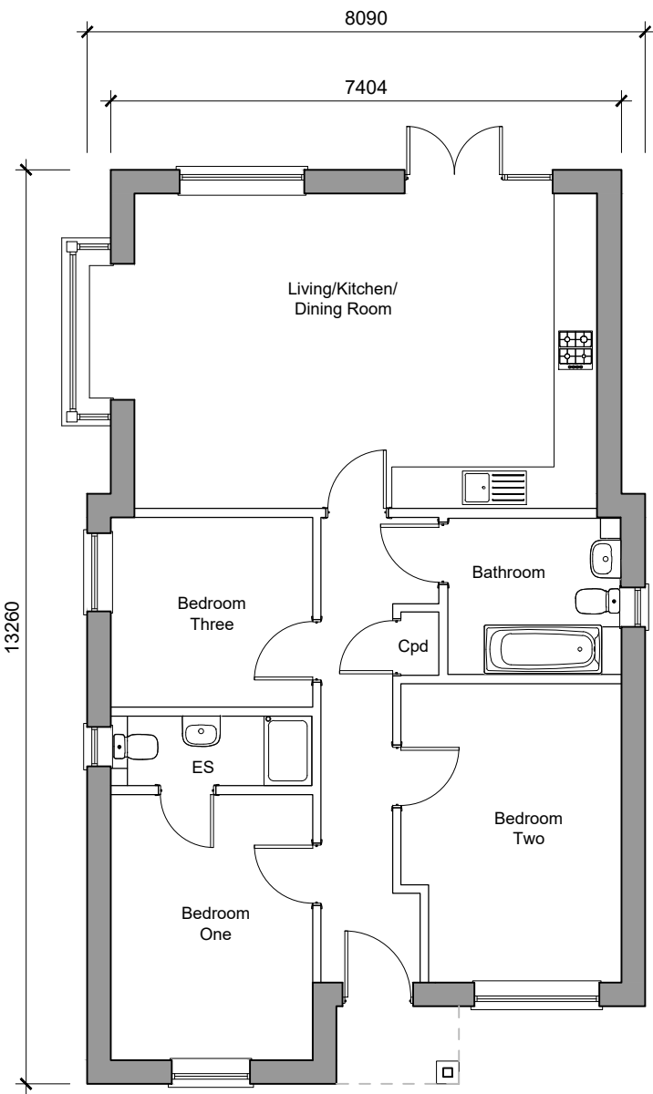
Type Bungalow Ground Floor Plan 3-Bedroom Bungalow 85.9sqm / 925sqft GIA (to finishes) Plots 84 Handed 64
