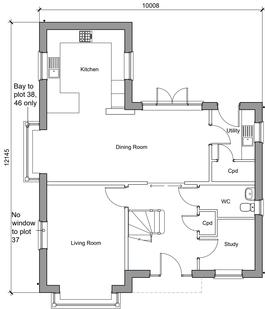
Type Maple Ground Floor Plan 4-Bedroom House 167.8sqm / 1806sqft GIA [to finishes] Plots 37, 41, 46 Handed 38
