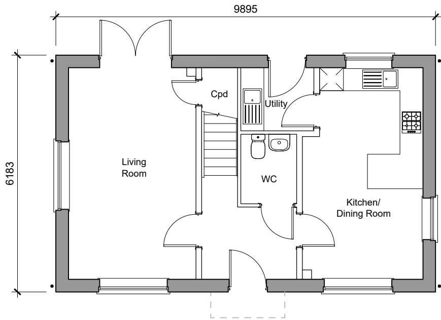
Type Spruce Ground Floor Plan 3-Bedroom House 102.1sqm / 1099sqft GfA [to finishes] Plots 10, 11
