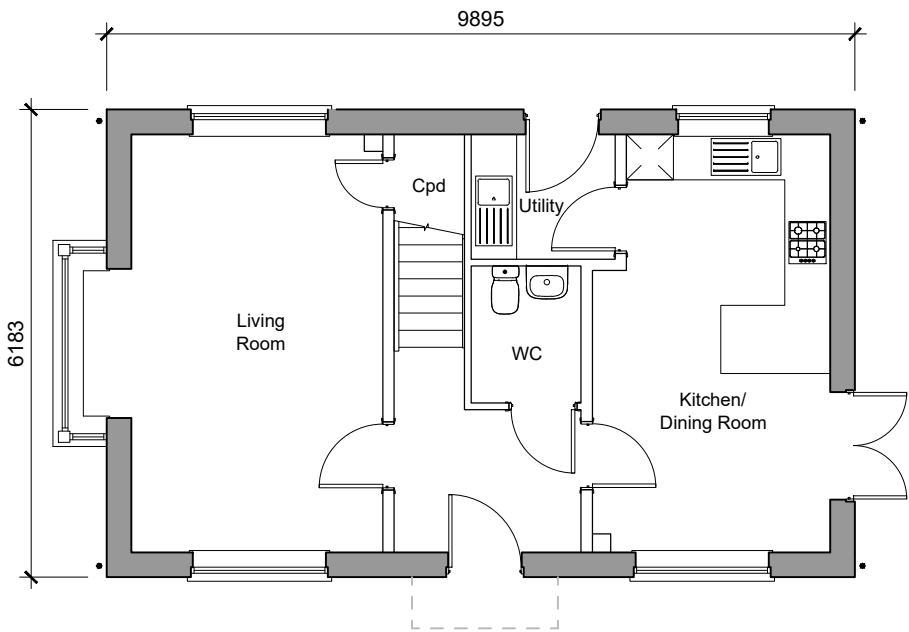
Type Spruce Ground Floor Plan
