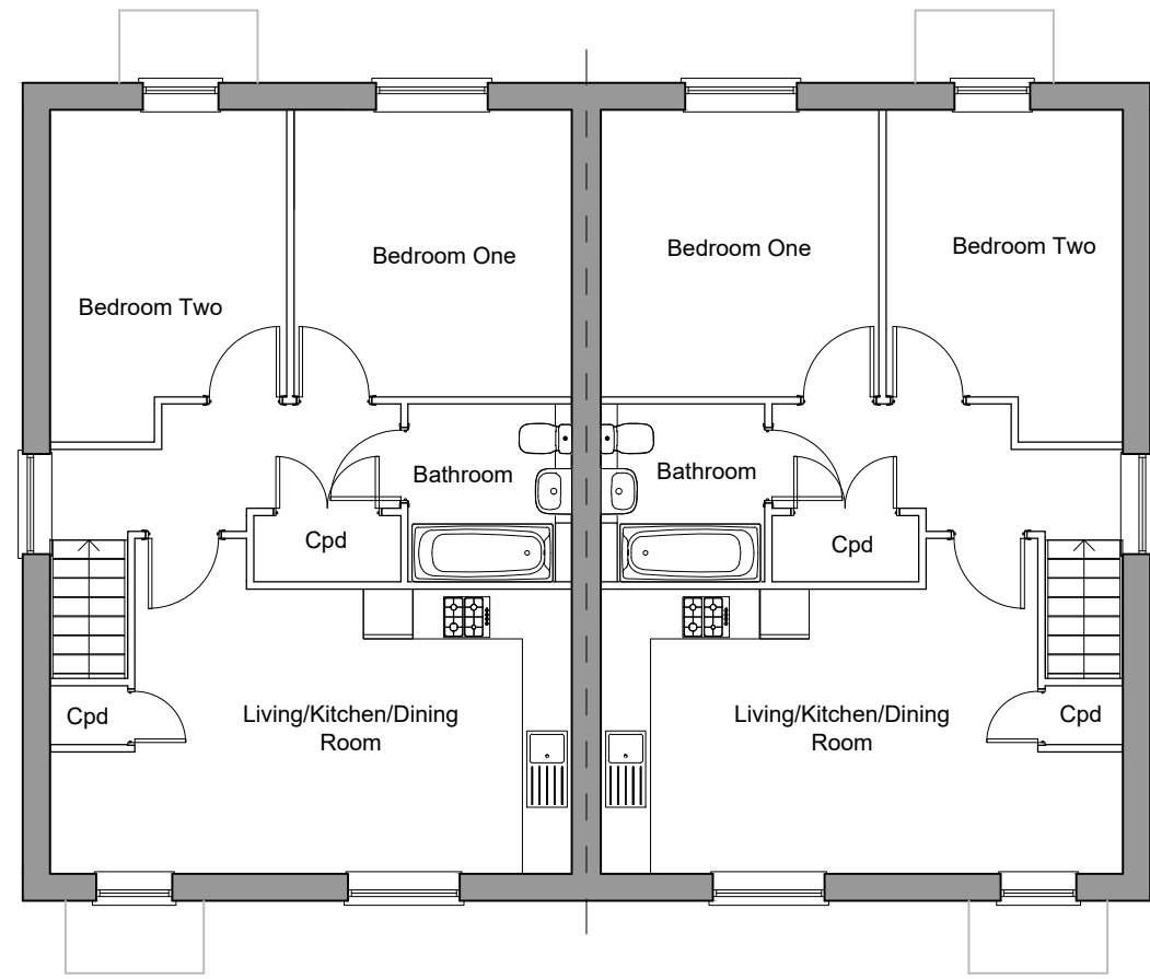
1st Floor Plan 2-Bedroom Flat 58.27sqm / 627sqft GIA [to finishes]
