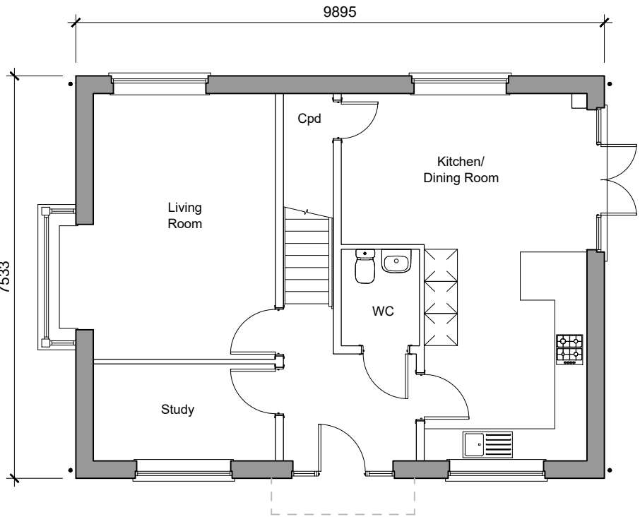
Type Chestnut Ground Floor Plan 4-Bedroom House 128.4sqm / 1382sqft GIA (to finishes) Plots 78
