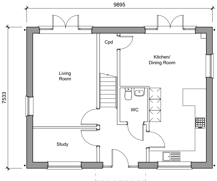
Type Chestnut Ground Floor Plan 4-Bedroom House 127.1sqm / 1368sqft GIA (to finishes) Plots 82
