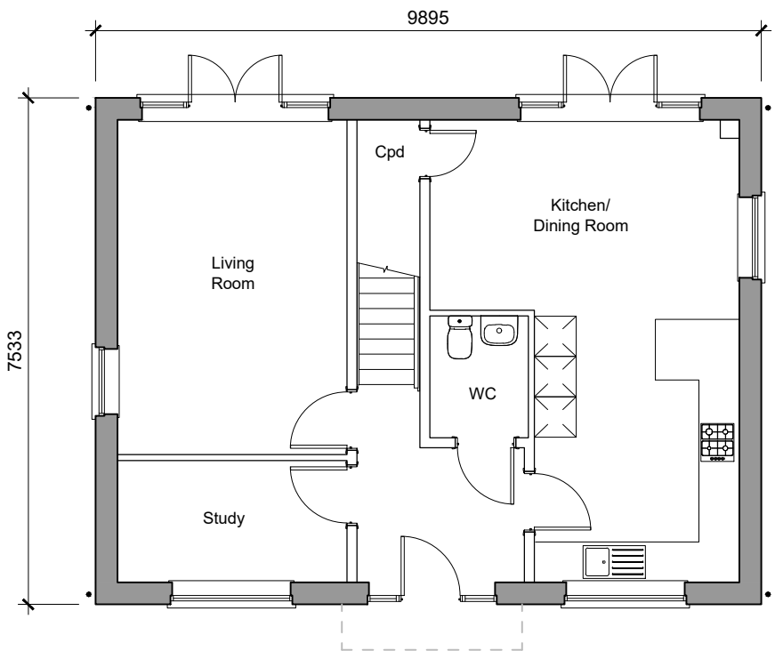
Type Chestnut Ground Floor Plan 4-Bedroom House 127.1sqm / 1368sqft GIA (to finishes) Plots 30, 36, 51, 58
