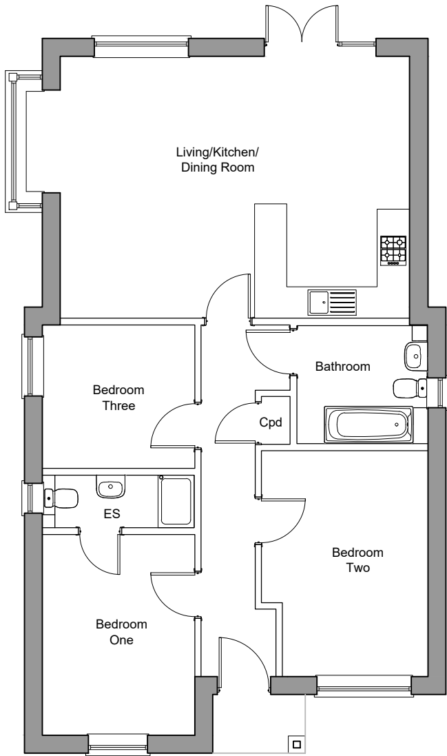
Type Bungalow Ground Floor Plan 3-Bedroom Bungalow 91.07sqm / 980sqft GIA [to finishes] Plots 84 Handed 64
