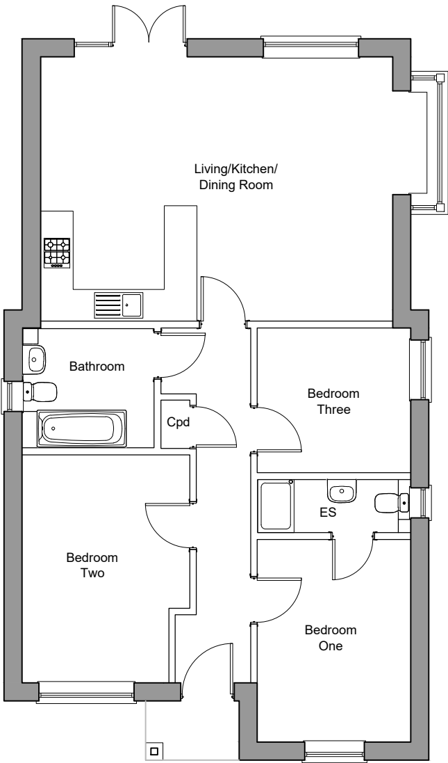
Type Bungalow Ground Floor Plan 3-Bedroom Bungalow 91.07sqm / 980sqft GIA [to finishes] Plots 83
