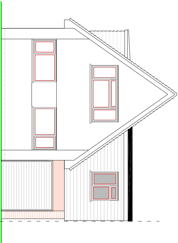
FRONT ELEVATION
