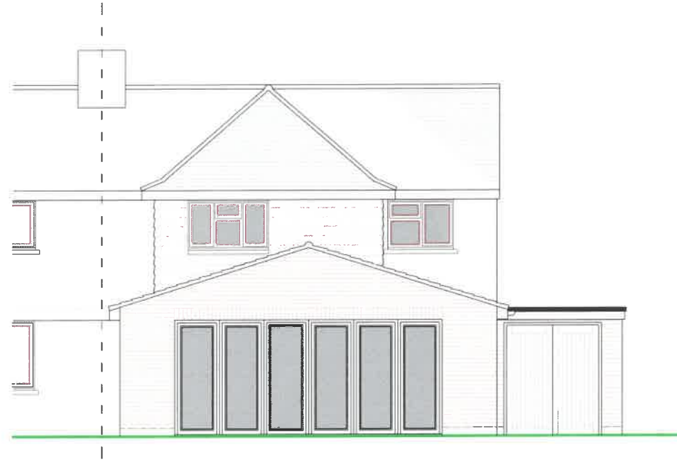
REAR ELEVATION
