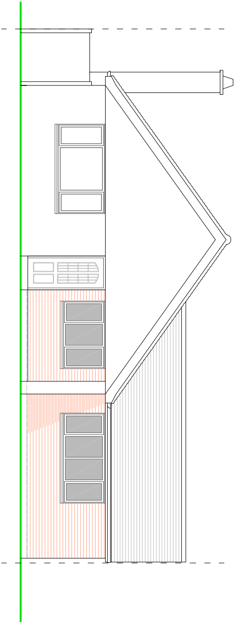
FRONT ELEVATION
