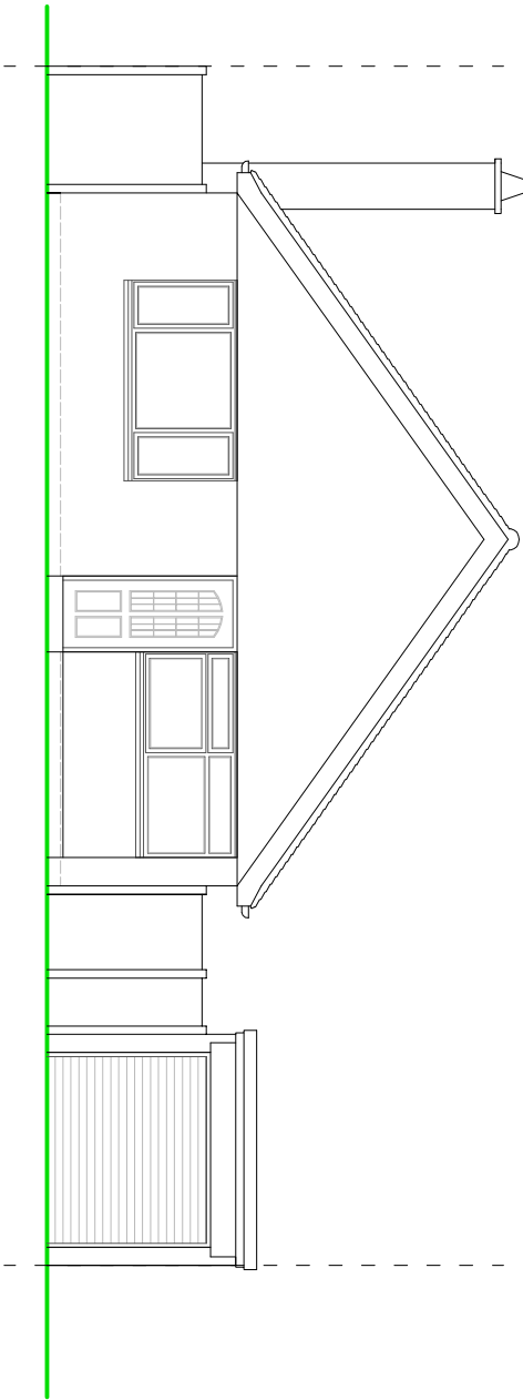
FRONT ELEVATION
